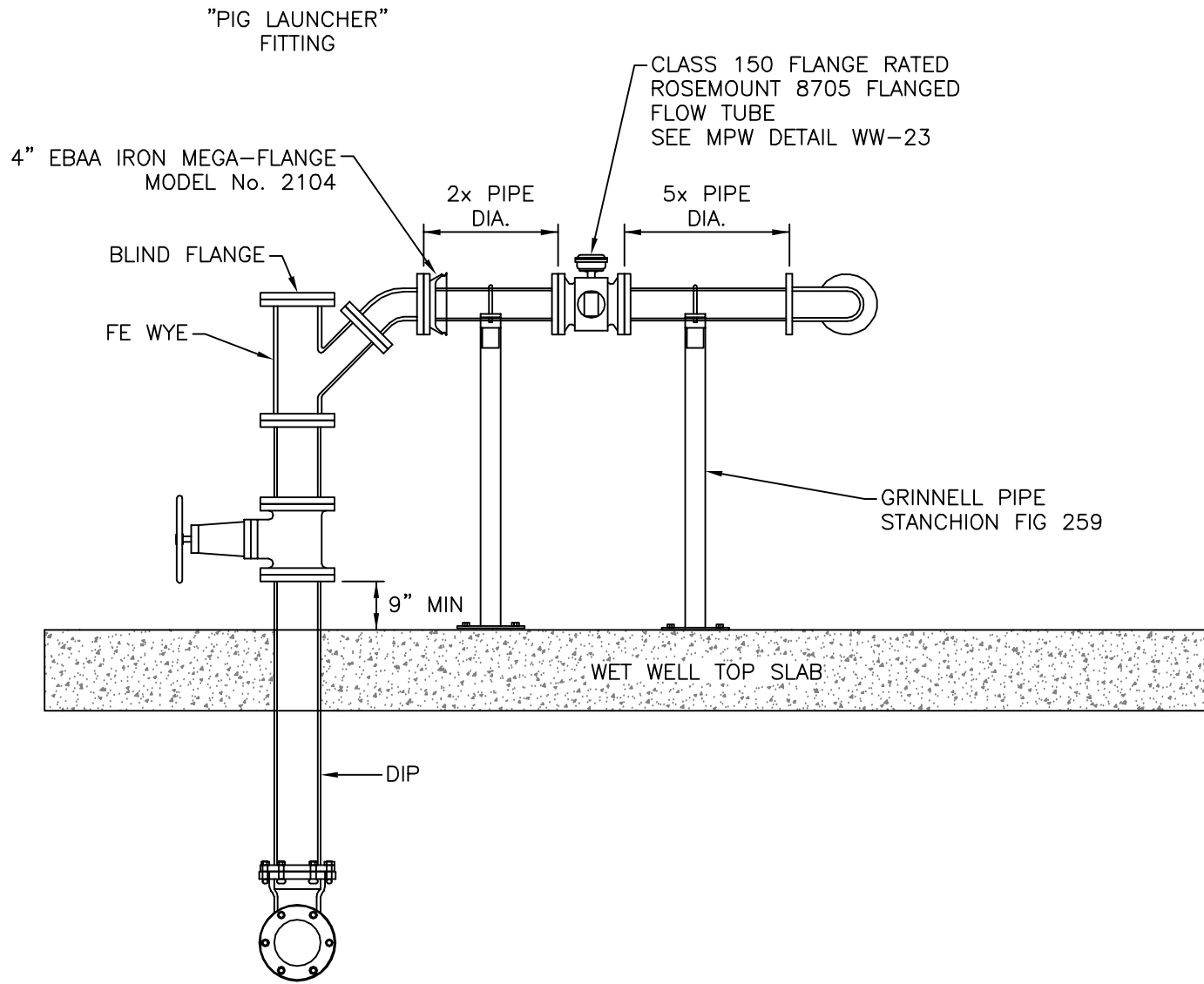
RISER SECTION
